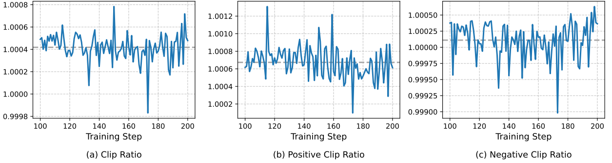
Figure 2: Curves of response-level IS ratios throughout DAPO training. The average IS ratios are shown in gray dashed lines.
