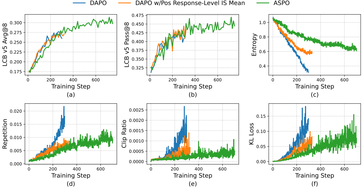
Figure 5: Comparison among DAPO, DAPO with response-level IS weights for positive samples, and ASPO. 图5：DAPO、采用响应级独立样本权重处理正样本的DAPO与ASPO的对比分析。
